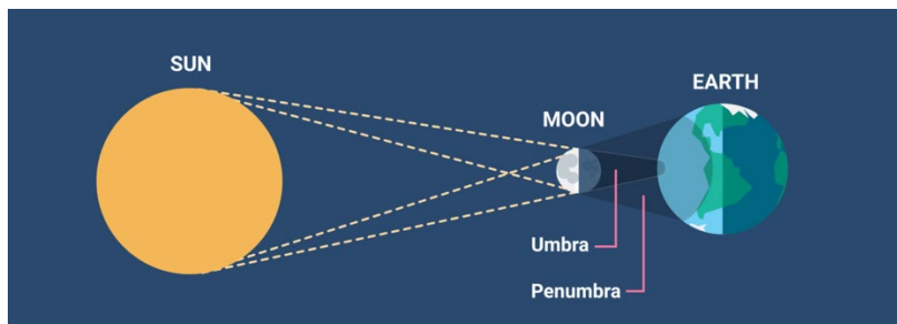
Figure 2: Figure 3: Mechanics of a total eclipse with umbral and penumbral shadows.
