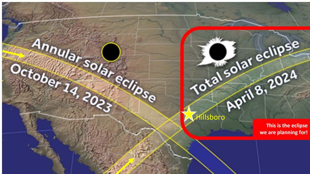
Figure 1: Paths of the annular and total solar eclipses crisscrossing over Texas. Source: Great American Eclipse .
